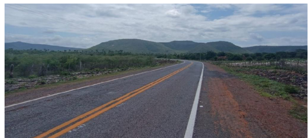
Figure 7. Hills and plateaus embedded in the reverse of the Ibiapaba. CE 232 in the area of Assemim, Viçosa do Ceará (CE).
